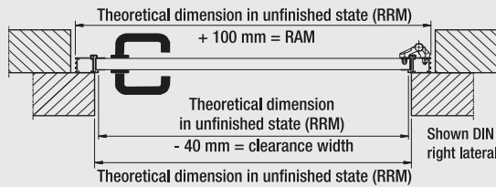
Installation behind the soffit, only inward opening
