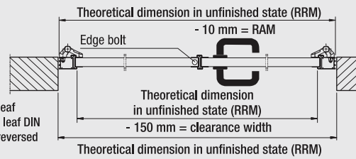
Caution: Frame outer dimension (RAM) = order size
