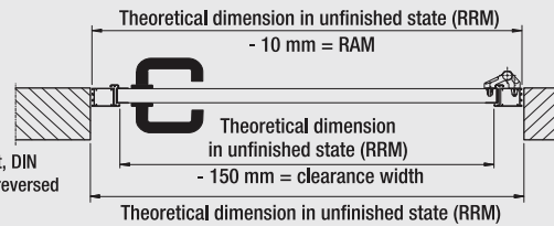
Installation within the soffit, inward or outward opening
