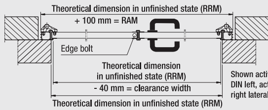
Installation behind the soffit, only inward opening
